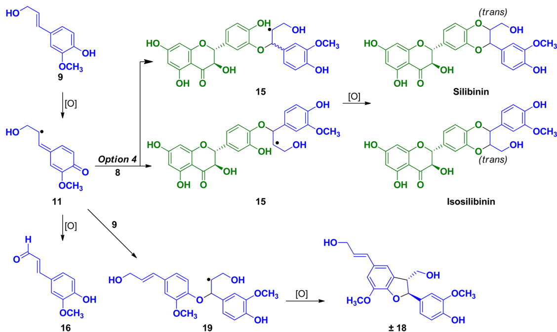
Scheme 6. Mechanistically Supported Biomimetic Synthesis of Flavonolignans
