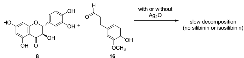
Scheme 6. Mechanistically Supported Biomimetic Synthesis of Flavonolignans
