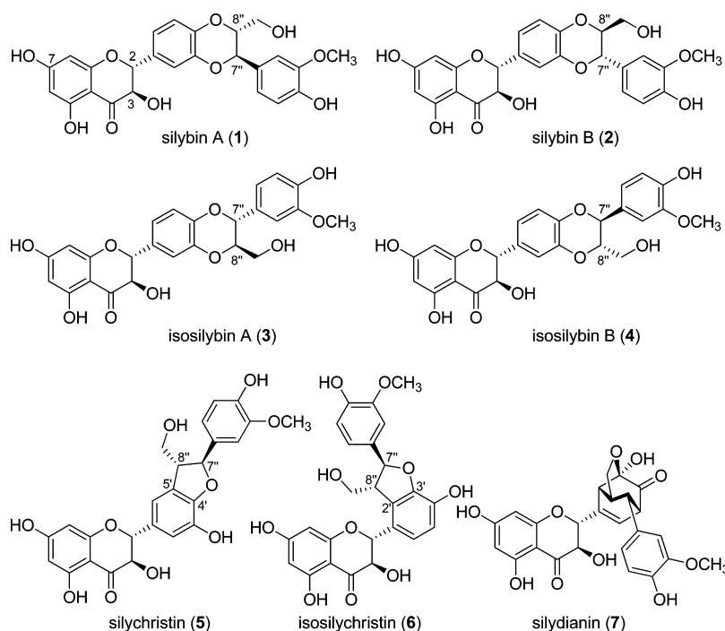
Figure 1. Flavonolignans from milk thistle; silybinin is a 1:1 mixture of 1 and 2, while isosilybinin is a 1:1 mixture of 3 and 4. 11
