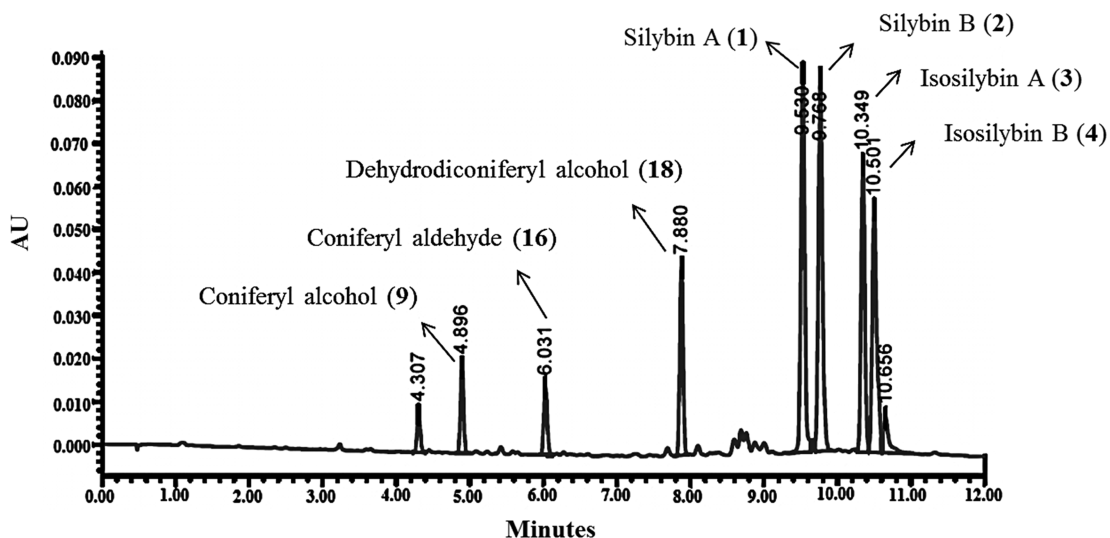
Figure 2. UPLC chromatogram of biomimetic reaction using conditions in Scheme 2. UPLC was conducted using a \text{CH}_3\text{OH}/\text{H}_2\text{O} (0.1% formic acid) gradient that was initiated at 5:95, increased to 50:50 over 10 min, and then held at that ratio for 2 min at a flow rate of 0.6 mL/min ( 50^\circ\text{C} ) using an HSST3 column monitored at 288 nm.
