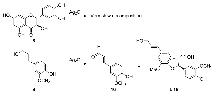
Scheme 4. Individual Oxidations of Taxifolin and Coniferyl Alcohol
