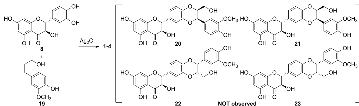
Scheme 4. Individual Oxidations of Taxifolin and Coniferyl Alcohol
